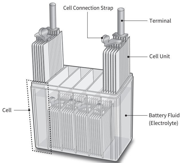
Battery internal components.
