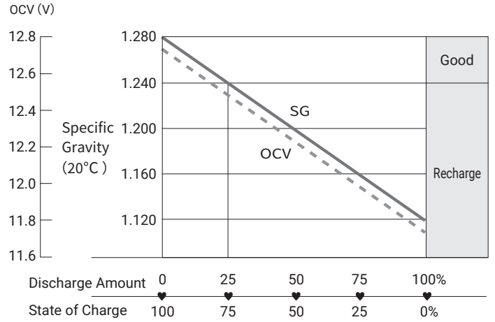
OCV vs State of Charge.
